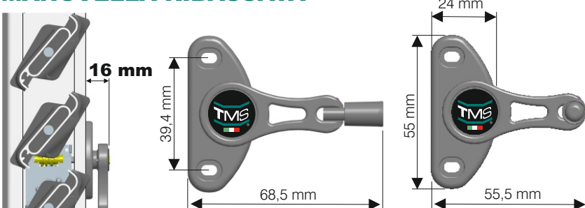
Sistema ROTARY con maniglia a manovella RIBASSATA ROTARY system version with manovella REDUCED handles
