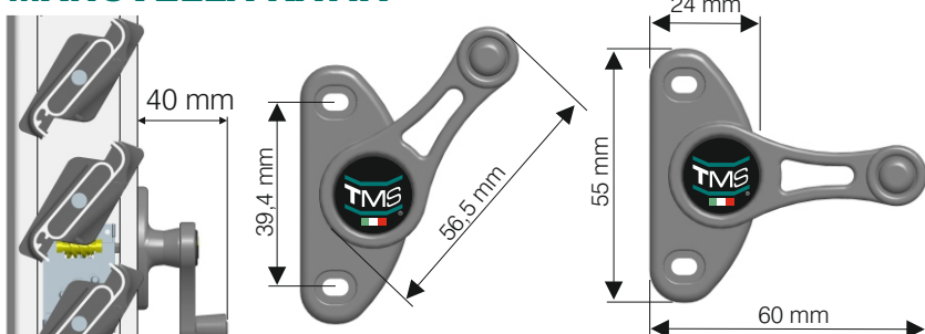
Sistema ROTARY con maniglia a manovella ROTARY system version with lever
